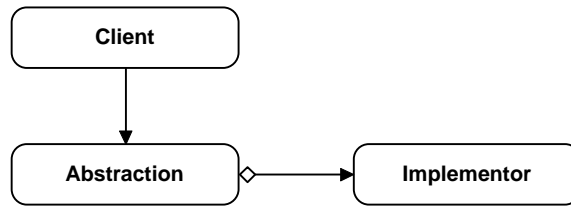
Figure 8-1: Role diagram of the Bridge pattern
