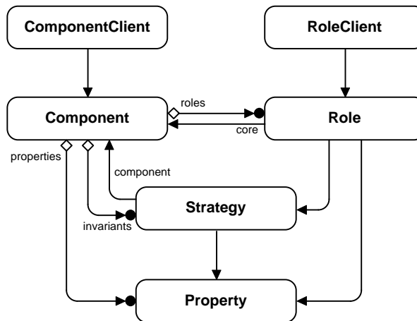
Figure 7-9: Role diagram of the Role pattern
